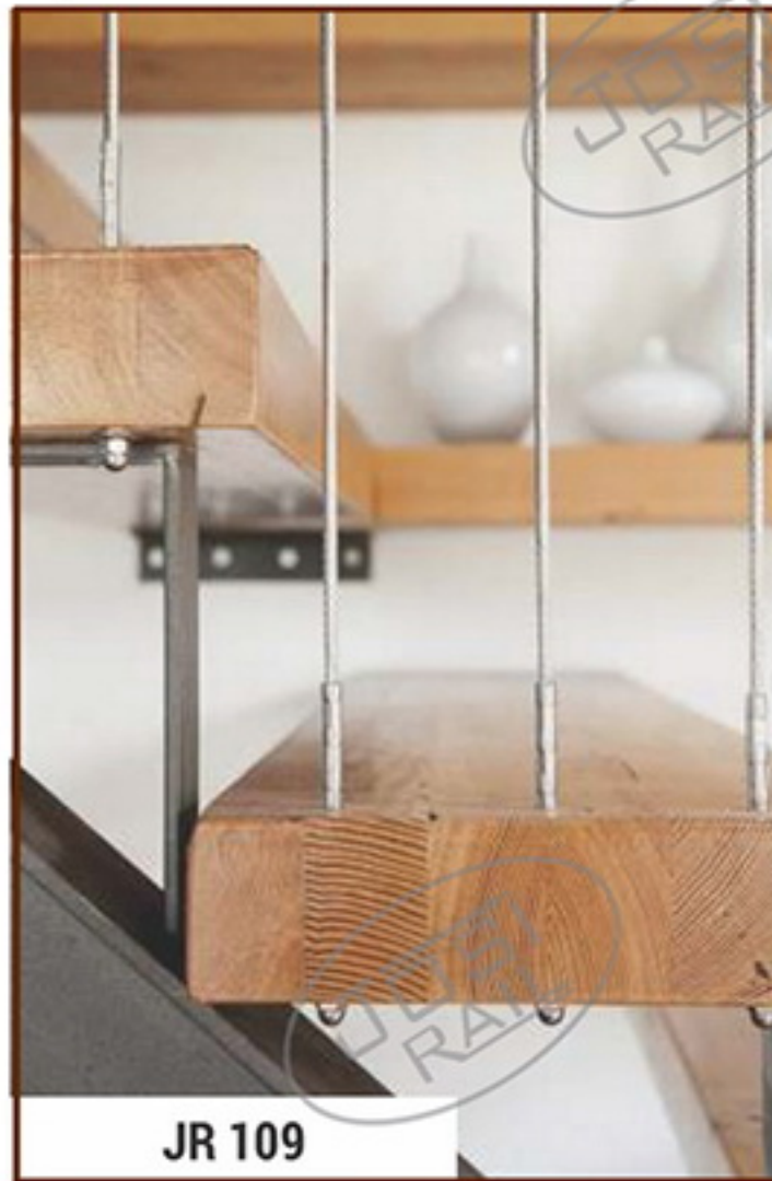
Wire Rope Staircase system
